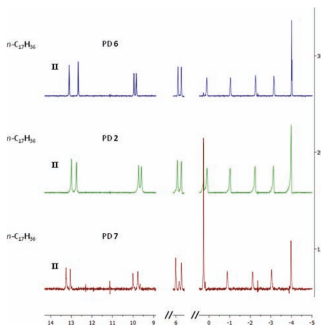
Figure 5. Comparison of the 1 H NMR spectra of assemblies containing either PD spacer unit 6, 2, or 7. These PD-units lack the ability to stack to the outside of the capsule and all form assembly II in the presence of n -heptadecane as guest.
