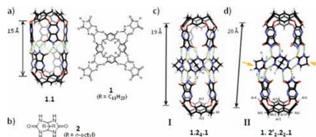
Figure 1. (a) Molecular model of dimeric capsule 1.1 , its approximate accessible cavity length and structure of cavitaund unit 1 . (b) Structure of propanediurea spacer unit 2 . (c) Molecular model of extended capsule I consisting of two cavitaund units 1 and four PD spacer units 2 , which are arranged in a “twisted-belt” fashion. (d) Molecular model of an isomeric capsule II again with two cavitaunds and four spacer units; In this case two PD units are oriented in a twisted fashion, while the remaining two PD units (marked by orange arrows) are bound horizontally with respect to the cavitaund. (Peripheral alkyl groups have been deleted for easier viewing.)
