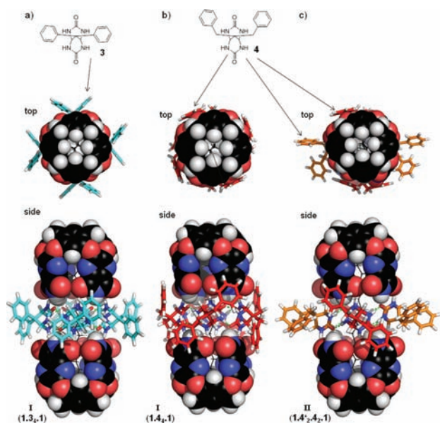
Figure 2. (a) Molecular models of assemblies I incorporating phenyl-PD 3 (cyan); (b) Model of assemblies I incorporating benzyl-PD 4 (red); (c) Model of assemblies II incorporating benzyl-PD 4 (marked red if oriented in a “twisted” fashion or marked orange if bound “horizontally” to the cavitand). The benzylic side chains of the PD 4 units bound in a “twisted” fashion (marked red) can fold back onto the surface of the capsule and give rise to potentially stabilizing \pi - \pi interactions with the assembly’s hydrogen-bonding array. (Peripheral alkyl groups have been deleted for easier viewing.)
